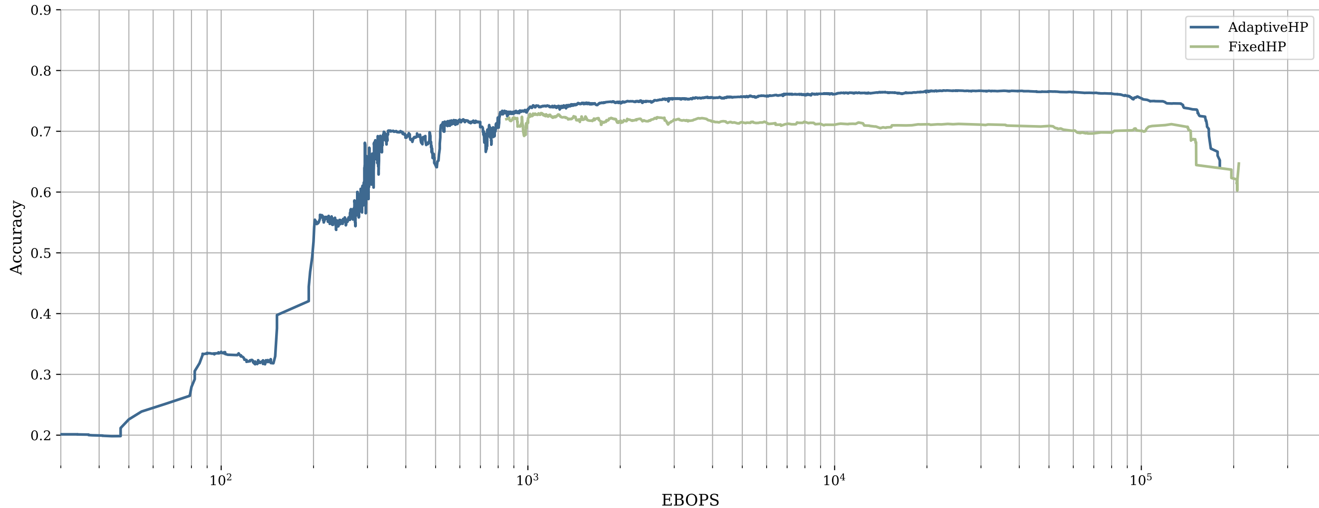
Jet Tagging HGQ: Accuracy over EBOPS (direct comparison, with averaging)
